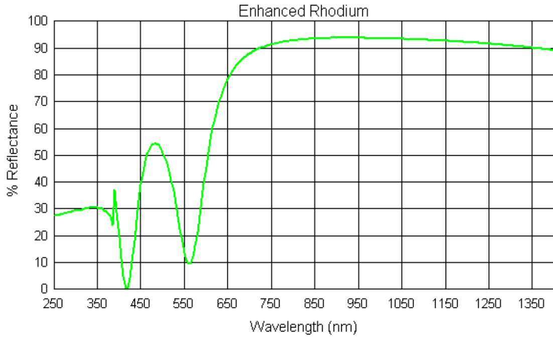
Fig.1: Enhanced Rhodium 700-1300
