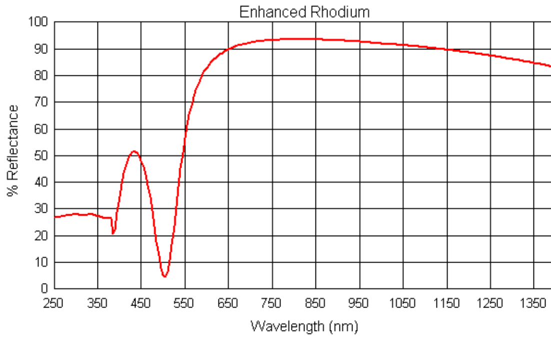
Fig.2: Enhanced Rhodium 650-1250
