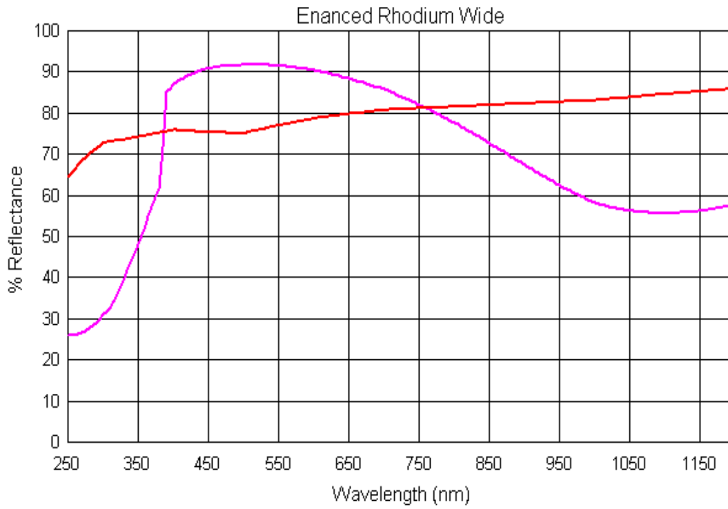
Fig.1: Reflectance of Enhanced Rhodium (Purple) vs. Rhodium (Red)
