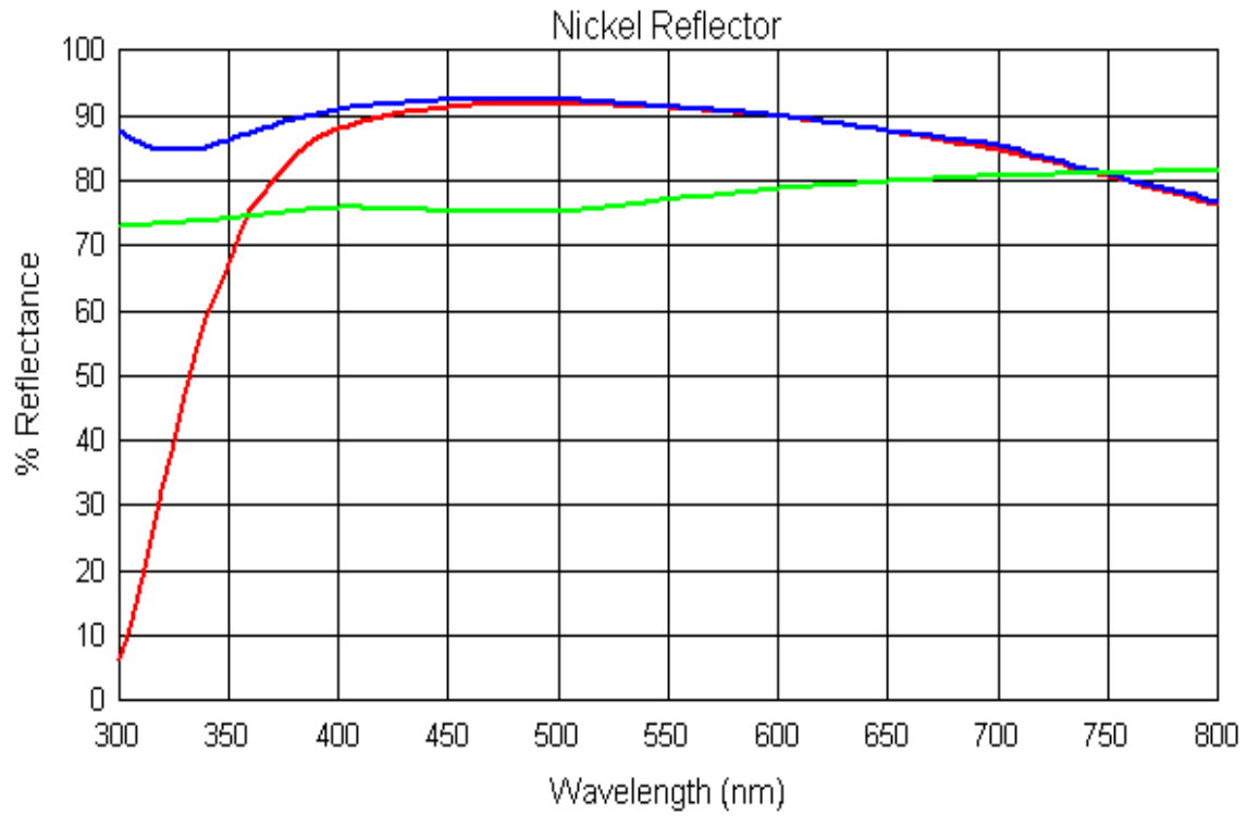
Fig.1: Reflectance of: Rhodium(Green); Protected Aluminum (Blue); Durable Enhanced Rhodium(Red)
