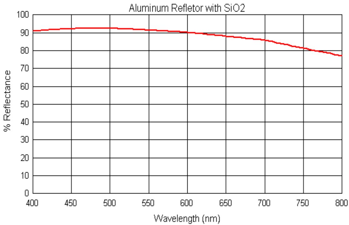
Fig.2: Nominal performance of a SiO 2 coated aluminum
