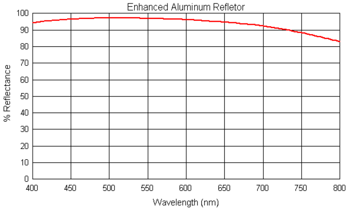
Fig.1: Nominal performance of a durable enhanced aluminum
