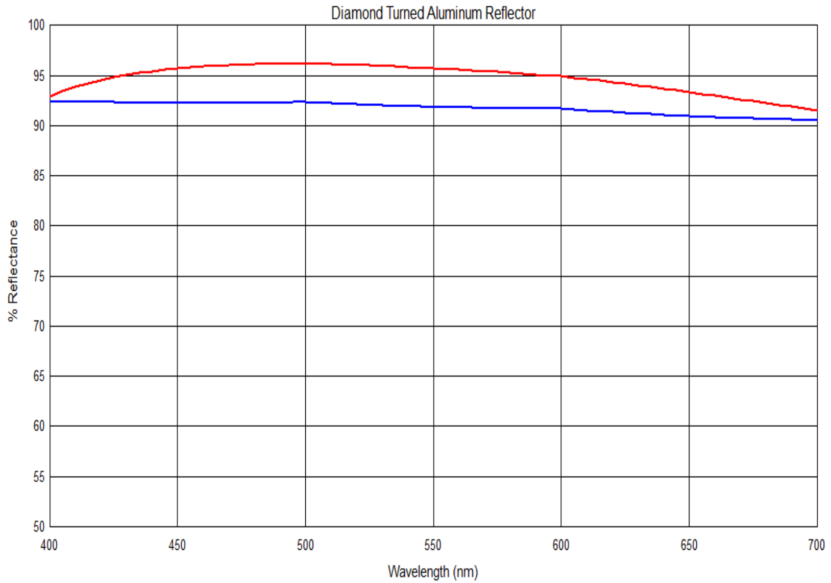
Fig.1: Reflectance of Diamond Turned Aluminum(Blue), and Enhanced Aluminum (Red) in the Visible
