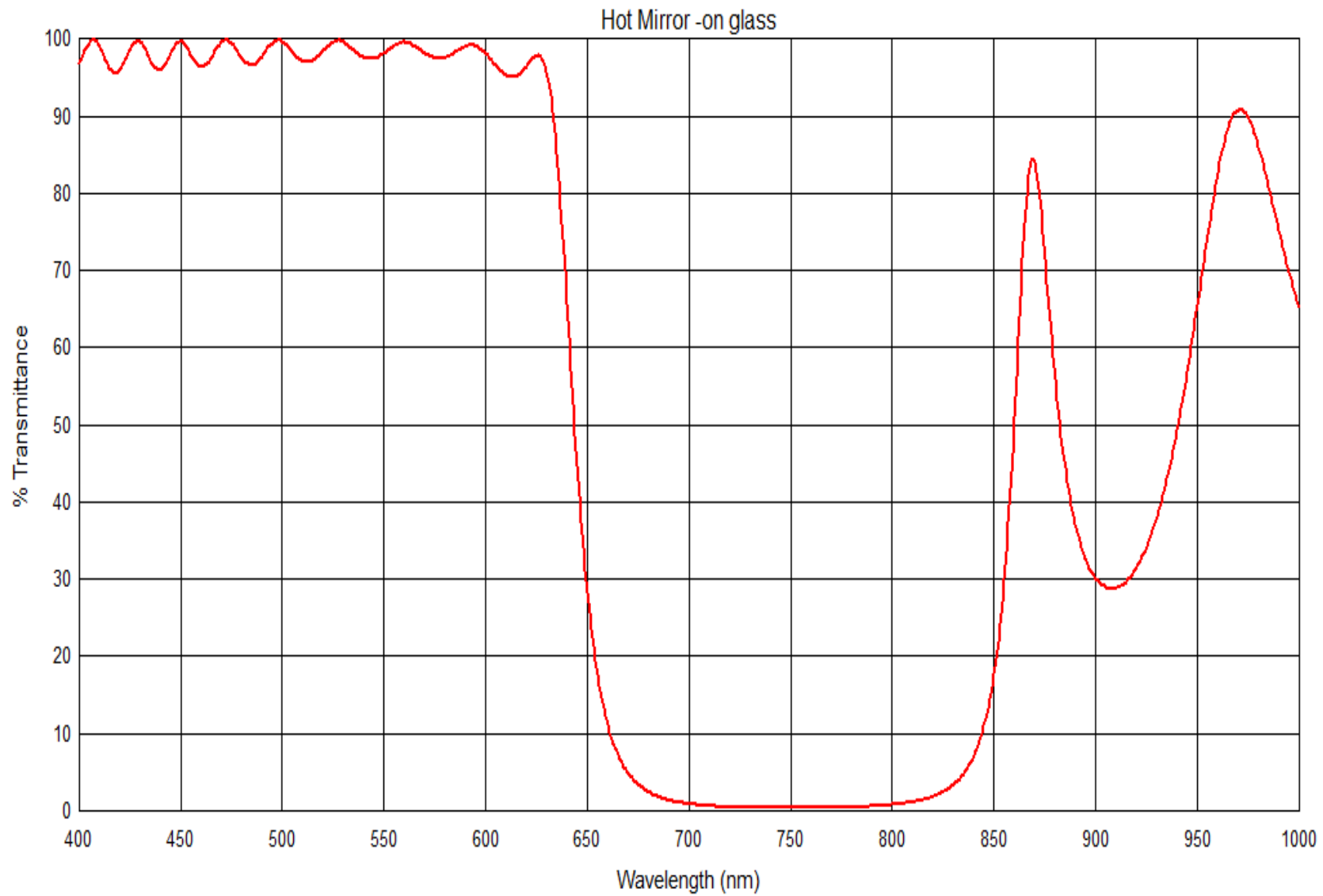
Fig.1: Nominal Performance of a Dielectric Hot Mirror on Glass
