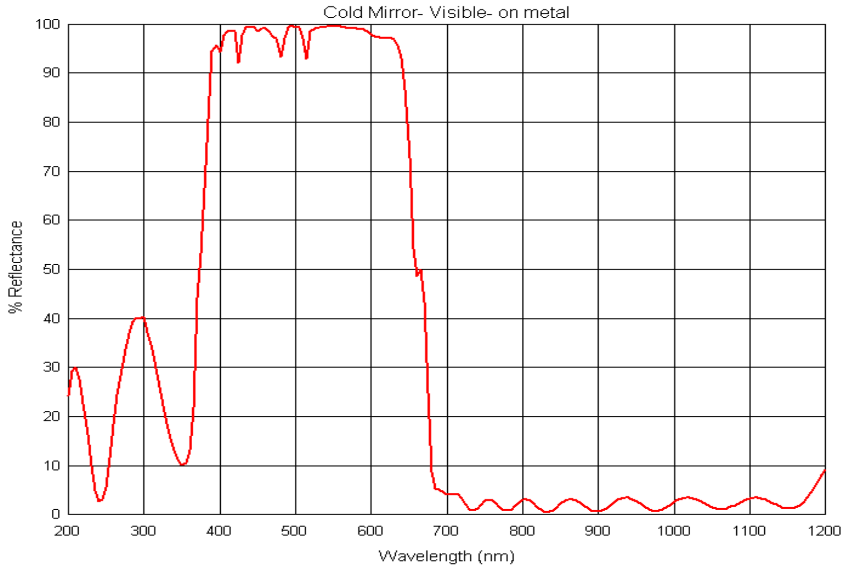
Fig.1: Nominal Reflectance of a Visible Cold Mirror on Metals
