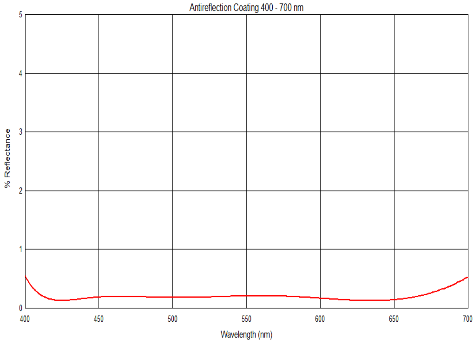
Fig.1: Nominal Performance of an AR coating in the Visible-All Oxide
