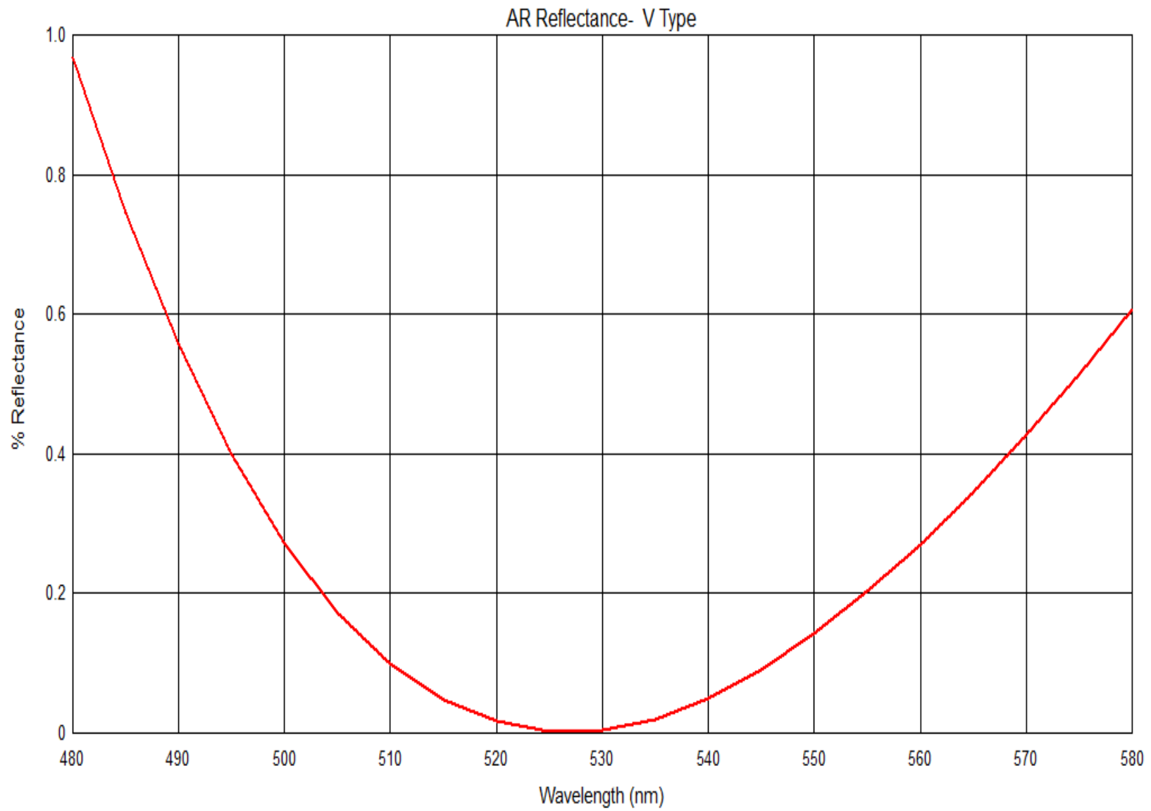
Fig.1: Nominal Performance of a V - Type AR coating -All Oxide
